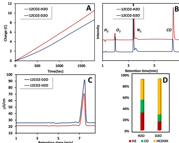
Fig. 3 CPE performed at -2.2 V vs. Fc^+/Fc^0 varying the heavier isotope of the proton source for 1/2 hour using a glassy carbon plate as the working electrode, Pt wire as the counter electrode and Ag/AgCl as the reference electrode. Charge consumption (A) followed by product detection using gas chromatography-TCD (B) and ion chromatography (C) and their faradaic yields (D) are compared for both H 2 O and D 2 O ( 12 CO 2 /H 2 O – red trace, 12 CO 2 /D 2 O – blue trace).
