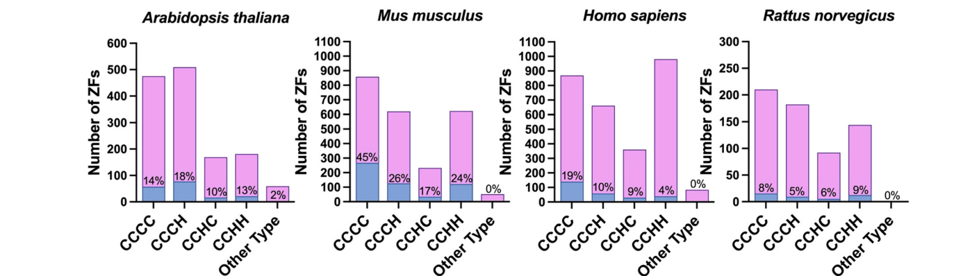
Fig. 4 (A) Pie-charts showing the types of ZFs that are persulfidated in each data set analyzed. ZFs are delineated based upon the number and composition of cysteine and histidine residues: CCCC, CCCH, CCHC, and CCHH. (B) Bar graphs displaying the number of each type of ZF present in each species analyzed (pink) compared to the number of persulfidated ZFs identified (blue). The percentage persulfidation is listed for each type of ZF.
