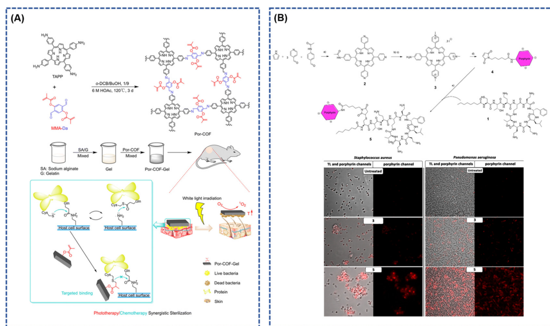
Fig. 10 (A) The design strategy and schematic of the Por-COF antibacterial nanoplatfrom; reproduced with permission of Ref. 104. Copyright © 2022, Wang, the Royal Society of Chemistry. (B) Synthetic Route of Cationic Porphyrin–Polymyxin B Conjugate (5) 9 , Scheme (a) Propionic acid, 3 h, 140 °C. (b) Iodomethane, anhydrous dimethylformamide (DMF), 1 h, 140 °C. (c) 25% TFA/H 2 O, 5 h, 100 °C. (d) 6-Maleimidohexanoic acid, HCTU, DIEA, anhydrous DMF, 24 h, RT. (e) PBS pH 6.5, 24 h, RT. And confocal laser scanning microscopy imaging of (left) S. aureus and (right) P. aeruginosa in different conditions: untreated and after incubation with 3 or 5. Reproduced with permission of Ref. 105. Copyright © 2017, Guern, American Chemical Society.
