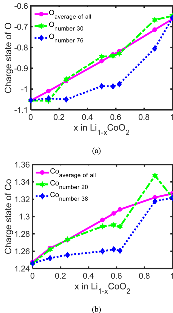
Fig. 5 The average charge states of all O, individual \text{O}_{\text{number}30} with surrounded Li extracted, and individual \text{O}_{\text{number}76} without surrounded Li extracted in \text{Li}_x\text{CoO}_2 during delithiation (a); the average charge states of all Co, individual \text{Co}_{\text{number}20} , and individual \text{Co}_{\text{number}38} in \text{Li}_x\text{CoO}_2 during delithiation (b).
