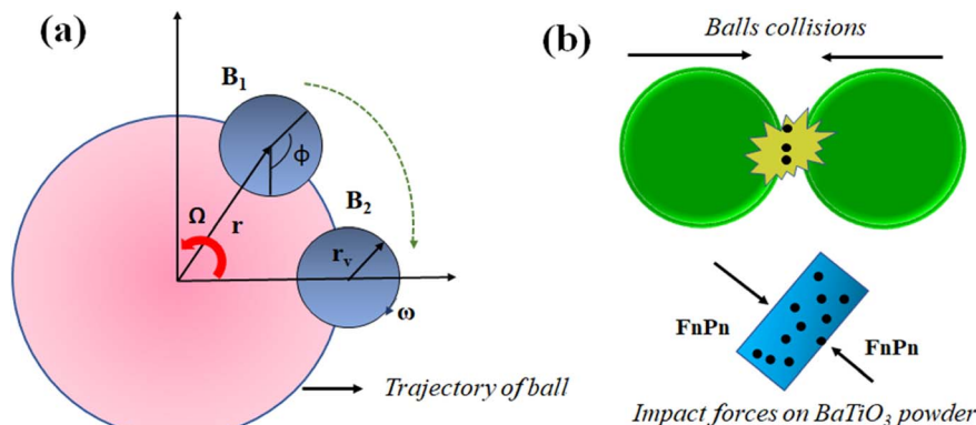
Fig. 10 (a) Trajectory of balls in planetary motion, (b) mechanics of balls for generating piezocatalysis in \text{BaTiO}_3 powder.
