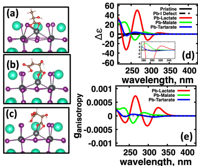
Fig. 6 Conformers bonded to excess \text{Pb}^{2+} on the \text{CsPbI}_3 cluster surface with the largest Boltzmann weights for (a) ( S )-lactate, (b) ( S )-malate, and (c) ( S,S )-tartaric acid. The color scheme for atomistic structures correspond to Cs (teal), Pb (grey), I (purple), O (red), C (brown), and H (white). (d) CD and (e) anisotropy spectra for the pristine \text{CsPbI}_3 cluster (black, solid), cluster with excess \text{Pb}^{2+} surface defect (black, dash-dot), ( S )-lactate (red), ( S )-malate (green), and ( S,S )-tartaric acid (blue) bonded to the surface \text{Pb}^{2+} site. The panel (d) inset shows the spectra near the optical gap. In panel (e), the black dashed line represents the zero level for reference.
