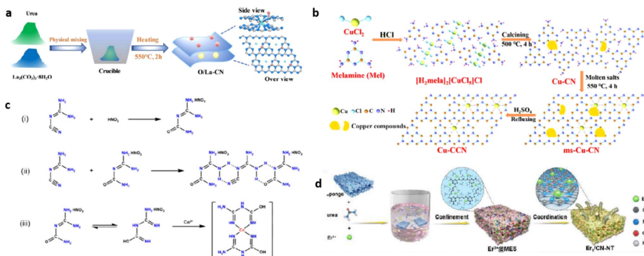
Fig. 6 (a) Template free direct synthesis of La single-atoms dispersed carbon nitride (O/La-CN). Reproduced with permission from ref. 16. Copyright 2020 American Chemical Society. (b) Direct synthesis of single Cu atoms supported crystalline g\text{-C}_3\text{N}_4 (Cu-CCN) through molten salts-reflux method. Reproduced with permission from ref. 18. Copyright 2020 American Chemical Society. (c) Mechanism of supramolecular preorganisation of g\text{-C}_3\text{N}_4 based cobalt SAC. Reproduced with permission from ref. 19. Copyright 2020 Elsevier. (d) Freeze drying assisted direct synthesis of erbium single atoms decorated g\text{-C}_3\text{N}_4 ( \text{Er}_1/\text{CN-NT} ). Reproduced with permission from ref. 9. Copyright 2020 John Wiley and Sons.
