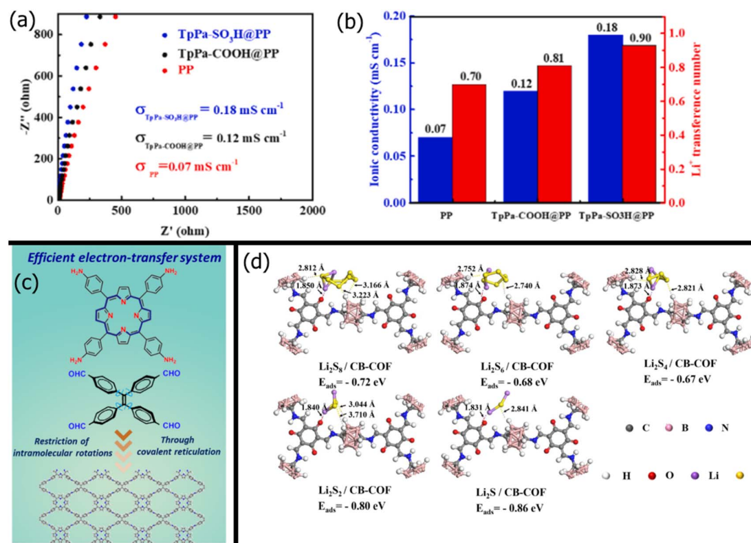
Fig. 10 (a) Ionic conductivity of the TpPa-SO 3 H@PP, TpPa-COOH@PP, and PP separators; (b) bar graph of ionic conductivity and Li-ion transference number of the TpPa-SO 3 H, TpPa-COOH, and PP separators 290 (Reproduced with permission from ref. 290. Copyright 2022, Elsevier). (c) Schematic showing the rigid structure of the TAPP-ETTB COF with an optimally designed electron transfer system via the porphyrin 292 (Reproduced with permission from ref. 292. Copyright 2022, The American Chemical Society). (d) Adsorption energies between the CB-COF molecule and various sulfur species ( \text{Li}_2\text{S}_x , 1 \leq x \leq 8 ) based on DFT calculation 289 (Reproduced with permission from ref. 289. Copyright 2021, The American Chemical Society).
