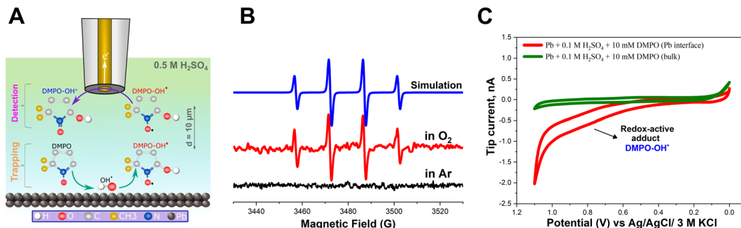
Fig. 3 Detection of [DMPO–OH]•. (A) Schematic for DMPO binding with OH• to produce [DMPO–OH]• which is then detected at the Au UME probe in an SG/TC SECM experiment. (B) ESR spectra recorded in 0.5 M H 2 SO 4 + 100 mM DMPO after soaking Pb–C anodes for 1 h in Ar and O 2 saturated conditions with the corresponding Easy Spin simulation fitting. (C) Cyclic voltammograms performed on the 12.5 μm Au UME probe from 0 to 1.1 V vs. Ag/AgCl/3 M KCl at a scan rate of 20 mV s -1 near the surface (10 μm) of Pb–C anode immersed in 0.5 M H 2 SO 4 + 10 mM DMPO and in the solution bulk (1000 μm).
