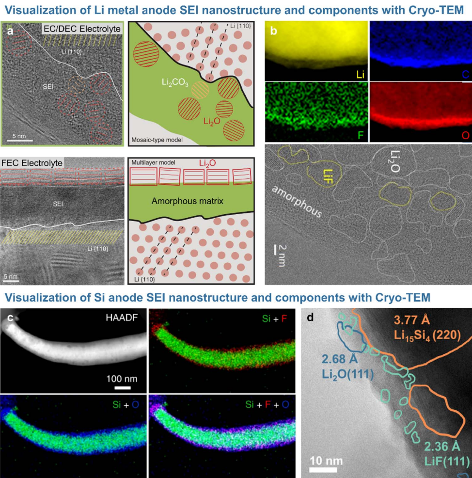
Fig. 3 (a) Cryo-TEM image of the SEI formed on lithium-metal with EC/DEC electrolyte and FEC electrolyte. Reproduced from ref. 17 with permission of AAAS, copyright 2017. (b) EELS mapping and Cryo-TEM images of the SEI on lithium-metal. Reproduced from ref. 18 with permission of Cell Press, copyright 2021. (c) Cryo-STEM image and EDS mappings of the silicon anode and SEI cycled in FEC-containing electrolyte. Reproduced from ref. 4 with permission of Springer Nature, copyright 2021. (d) Cryo-TEM image of the silicon anode after a cycle. Reproduced from ref. 19 with permission of Cell Press, copyright 2021.
