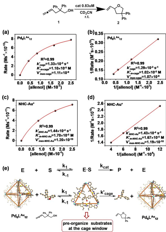
Fig. 6 Kinetic experiments and implications in the cyclization reaction of allenol 1 . (a) Kinetic analyses and (b) Lineweaver–Burk plot for the \text{Pd}_6\text{L}^{\text{Au}}_{12} cage. (c) Kinetic analyses and (d) Lineweaver–Burk plot for \text{NHC-Au}^+ . (e) The formula of the Michaelis–Menten model and the \text{Pd}_6\text{L}^{\text{Au}}_{12} cage (using the SCXRD structure as the model) exhibits the features of enzymatic catalysis in the cyclization of allenol. Color coding: C: gray; N: dark blue; Au: yellow; Pd: light blue; O: red; H: white.
