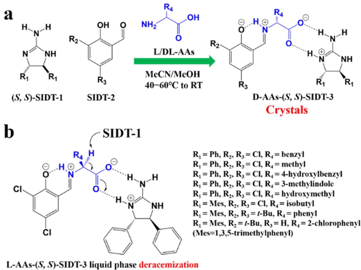
Fig. 21 (a) Substrates for SIDT strategy of L to D conversion and deracemization. (b) Acid/base catalysis-based mechanism for L-AA-( S,S )-SIDT-3 racemization (or DL-AAs deracemization). 40
