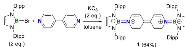
Scheme 1 Synthesis of 1 .
