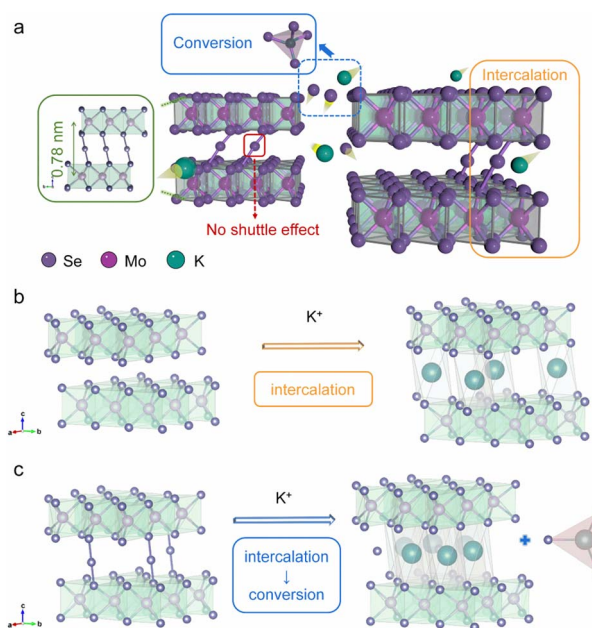
Fig. 1 (a) Schematic illustration of the modulation of Se–Se bonds. (b and c) Crystal structure and mechanism of \text{MoSe}_2 and \text{MoSe}_{2+x} , respectively. Purple atoms represent selenium, pink atoms represent molybdenum, and green atoms represent potassium.
