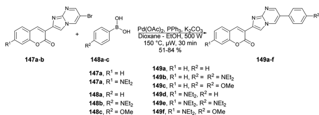
Scheme 53 Synthesis of 6-aryl-2-coumarin-3-yl-imidazopyrimidines 149a-f .
