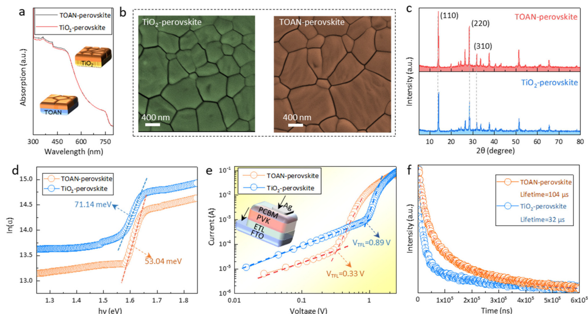
Fig. 2 Perovskite films grown on \text{TiO}_2 and TOAN substrates. (a) The UV-vis absorption patterns of the perovskite films grown on \text{TiO}_2 and TOAN layers. (b) SEM images and (c) XRD patterns of the \text{TiO}_2 - and TOAN-perovskite, respectively. (d) The h\nu versus \ln(\alpha) for the \text{TiO}_2 - and TOAN-perovskite films. The E_u can be obtained from the following equation: \alpha = \alpha_0 \exp(E/E_u) , where \alpha_0 is a constant. (e) The SCLC curves of the \text{TiO}_2 - and TOAN-devices; the inset exhibits the device structure. (f) Transient photovoltage decay curves for the \text{TiO}_2 - and TOAN-perovskite films.
