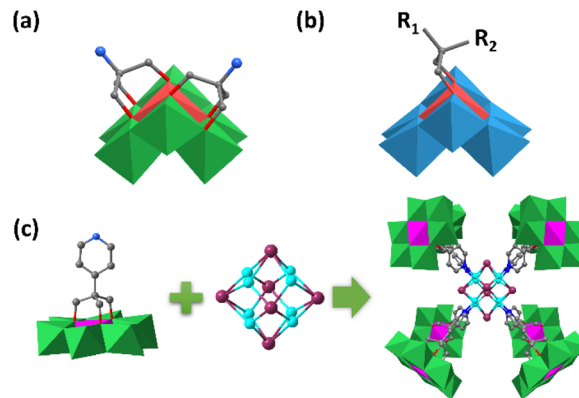
Fig. 5 (a) Schematic diagram of the \{[H_3NC(CH_2O)_3]_2MnMo_6O_{18}\}^{6-} structure. (b) Schematic diagram of the \{[R_1R_2C(CH_2O)_2]Mn^{IV}W_6O_{22}\}^{6-} structure. (c) Synthesis diagram of [TBA]_{14}[Cu_8I_6][HCr(OH)_3Mo_6O_{18}L_3]_8 . Color code: {MoO 6 }, green octahedron; {MnO 6 }, red octahedron; {WO 6 }, blue octahedron; {CrO 6 }, pink octahedron; C, gray; N, light blue; Cu, turquoise; I, purple.
