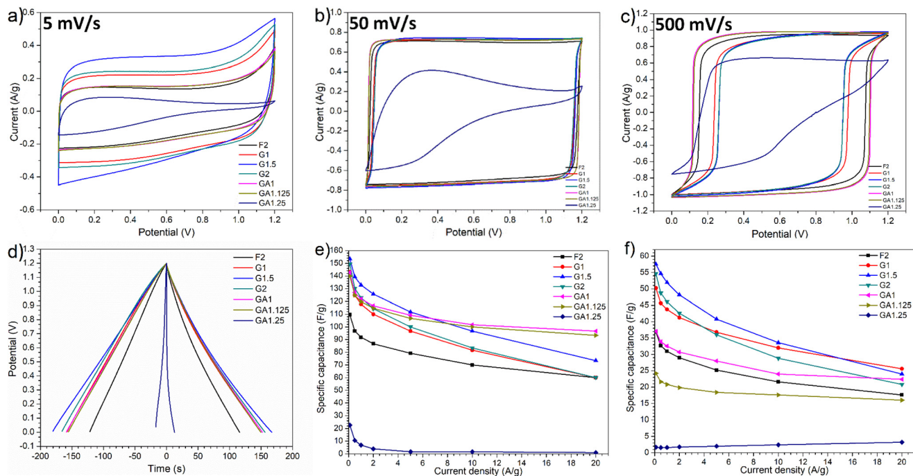
Fig. 4 Electrochemical performance of MC electrodes: (a–c) CV test at scan rates of 5, 50, and 500 mV s^{-1} , (d) galvanostatic charge/discharge at 0.5 A g^{-1} , (e) gravimetric capacitance in 6 M KOH electrolyte; (f) gravimetric capacitance in [N_{2220}][NTf_2]/ACN electrolyte.
