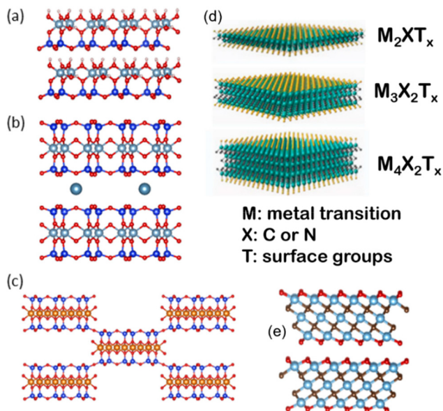
Fig. 2 Crystal structures of a selection of clay minerals (a–c) based on Al- and Mg- phyllosilicates of 1:1 type such as kaolinite (a), 2:1 type such as montmorillonite (b) and sepiolite (c), and 2D MXenes (d and e) of M_{n+1}X_nT_x , as a general formula (M = early transition metal; X = C and/or N, and T_x = OH, F surface terminations) (d). The value n = 1-4 indicates the number of transition metal layers (and carbon and/or nitrogen layers), i.e., Ti_3C_2T_x ( n = 2 ) (e). The (a), (b), (c) and (e) figures have been built using VESTA 3 software, 33 and (d) has been adapted from Wyatt et al. , 2D MXenes: Tunable Mechanical and Tribological Properties, Adv. Mater. , 2021, 33, 2007973, Wiley.
