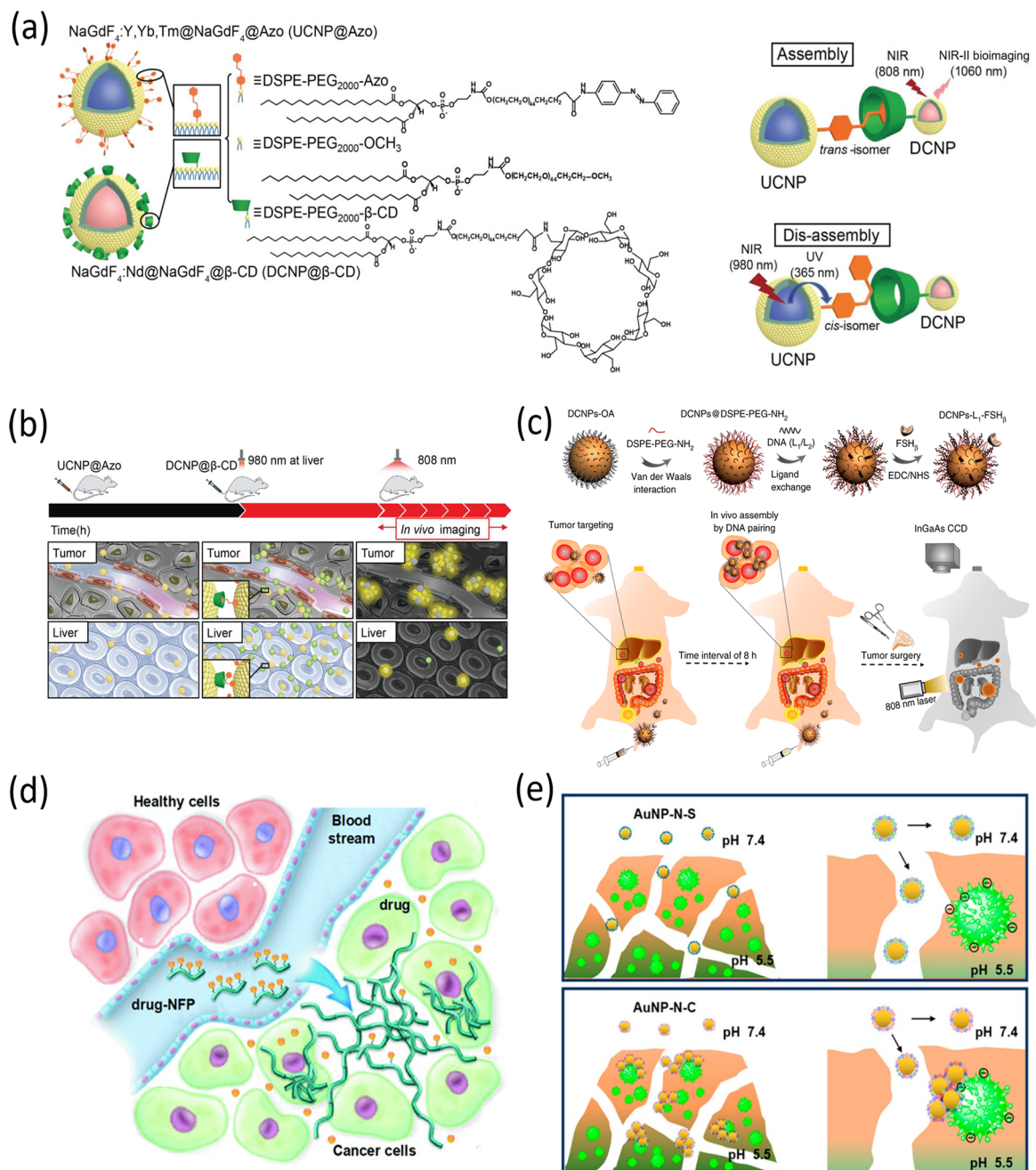
Fig. 4 (a) Preparation of azobenzene (Azo) modified \text{NaGdF}_4:10\% \text{Y}, 25\% \text{Yb}, 0.5\% \text{Tm} @ \text{NaGdF}_4 (UCNP@Azo) and \beta -CD modified \text{NaGdF}_4:5\% \text{Nd} @ \text{NaGdF}_4 (DCNP@ \beta -CD). 42 Reproduced from ref. 42 with permission from Wiley-VCH GmbH, copyright 2018. (b) In vivo assembly of UCNP@Azo and DCNP@ \beta -CD with improved tumor targeting. 42 Reproduced from ref. 42 with permission from Wiley-VCH GmbH, copyright 2018. (c) Schematic illustration of the stepwise preparation of DNA and FSH \beta modified DCNPs (DCNPs-L1-FSH \beta ) and in vivo assembly of DCNPs-L1-FSH \beta (first injection) and DCNPs-L2-FSH \beta (second injection) with improved tumor targeting and rapid hepatic and renal clearance after two-stage in sequence injections. 86 Reproduced from ref. 86 with permission from Springer Nature, copyright 2018. (d) NFP has a high aspect ratio that promotes its take up by solid tumors. Multiple NFPs can penetrate tumor tissue and subsequently transform into larger interfibril networks via in situ activation by tumor-associated proteases, thus minimizing lymphatic clearance. 89 Reproduced from ref. 89 with permission from Wiley-VCH GmbH, copyright 2018. (e) AuNP-N-S, with negatively charged surfaces, dispersed stably in MRSA biofilm and healthy tissues but with no bactericidal effect under NIR light irradiation; AuNP-N-C, with positively charged surfaces in acidic MRSA biofilm (pH \sim 5.5), effectively adhered to bacteria and rapidly aggregated in MRSA biofilm, exhibiting great bactericidal effect under NIR light irradiation without damage to surrounding healthy tissues (pH \sim 7.4). 92 Reproduced from ref. 92 with permission from the American Chemical Society, copyright 2017.
