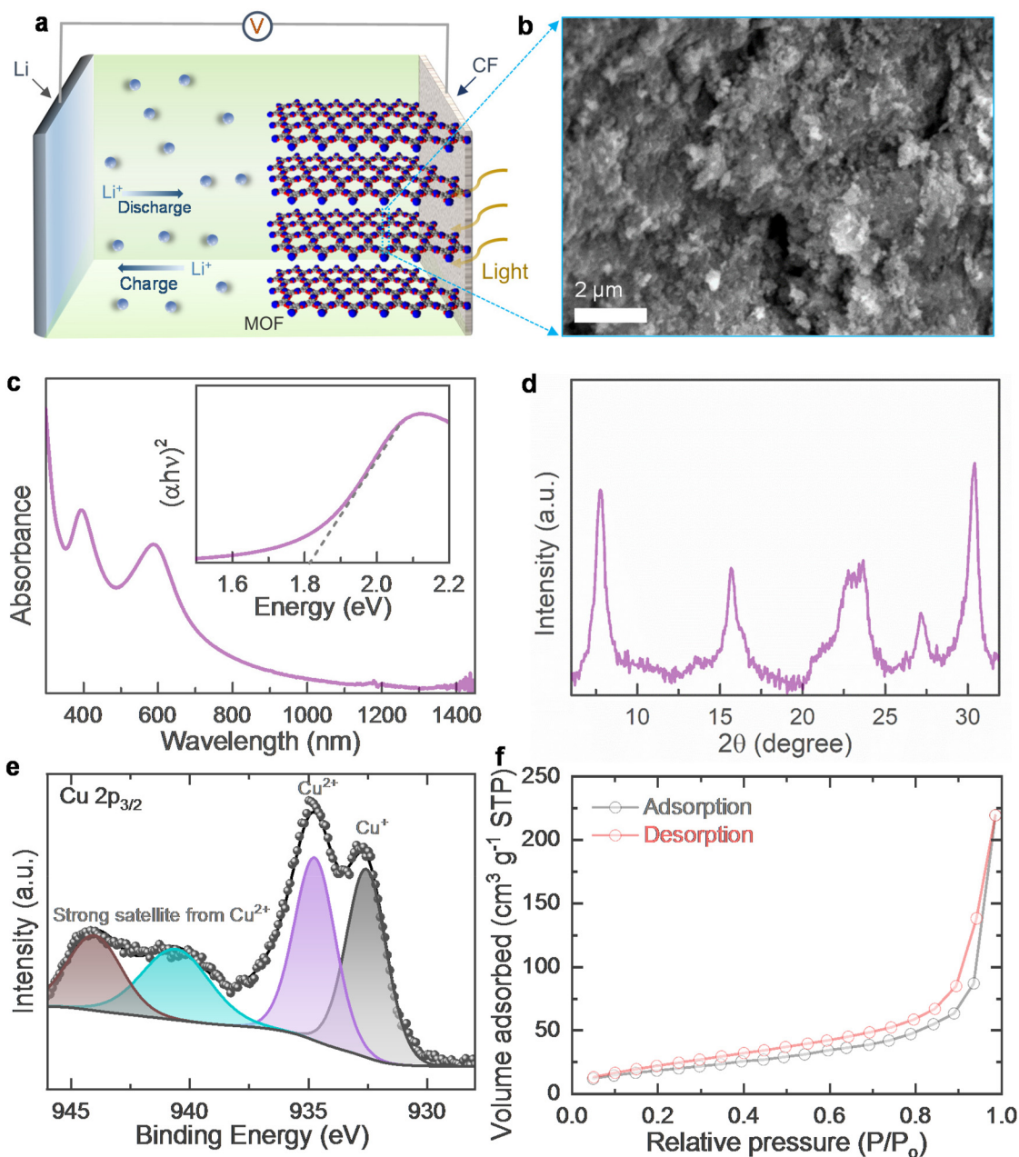
Fig. 1 (a) Schematic illustration of Ph-LIB using Cu-HHB photo-cathode and Li counter electrode. (b) SEM image of the Cu-HHB MOF. (c) UV-Vis absorption spectrum of Cu-HHB: the Tauc plot (inset) shows the absorption edge energy of \sim 1.81 eV. (d) PXRD pattern of Cu-HHB, with diffraction peaks at 2\theta \sim 7.8^\circ , 15.7^\circ , 27.2^\circ and 30.2^\circ can be indexed to (100), (200), (300) and (001) planes. The broad peak at 2\theta \sim 22\text{--}24.2^\circ could be attributed to the glass substrate. (e) High-resolution XPS scan of Cu 2p_{3/2} of Cu-HHB. (f) BET N_2 adsorption isotherms of Cu-HHB.
