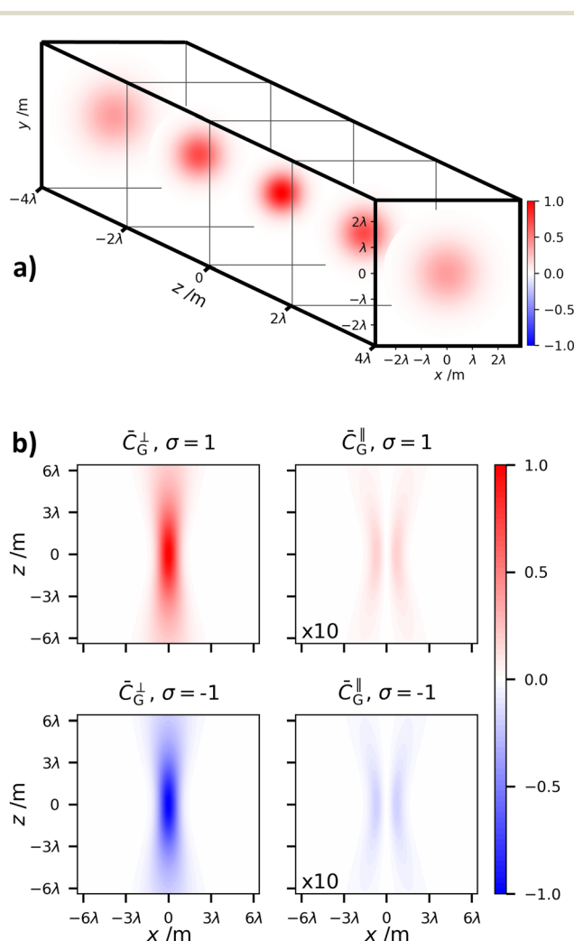
Fig. 2 (a) 3D plot showing the variation of \bar{C}_G for a beam with \sigma = 1 along the propagation axis. (b) 2D plot showing both the diffractive properties of the transverse contribution \bar{C}_G^\perp (left) and the longitudinal contribution \bar{C}_G^\parallel (right) to \bar{C}_G for \sigma = \pm 1 , normalised to the total \bar{C}_G . In all plots w_0 = \lambda .
