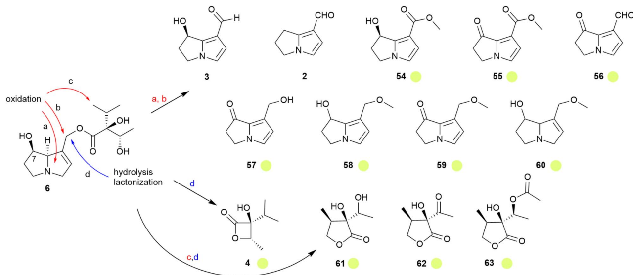
Fig. 11 Transformations of lycopsamine ( 6 ) into volatile dehydropyrrolizines and necic acid lactones, adopted from Schulz et al. 54 The colour code indicates occurrence only in tribe (•). Reprinted by permission from Elsevier: Biochemical Systematics and Ecology , Semicheicals derived from pyrrolizidine alkaloids in male ithomiine butterflies (Lepidoptera: Nymphalidae: Ithomiinae), S. Schulz, Copyright (2004). 54
