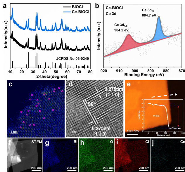
Fig. 1 Structural characterization. (a) XRD patterns of BiOCl and Ce-BiOCl. (b) High-resolution Ce 3d XPS spectra of Ce-BiOCl. Atomic resolution HAADF-STEM images of (c) Ce-BiOCl. (d) HRTEM image of Ce-BiOCl. (e) AFM images and corresponding height profiles of Ce-BiOCl. (f) STEM image of Ce-BiOCl and (g)–(j) the corresponding elemental distribution of Bi, O, Cl and Ce.
