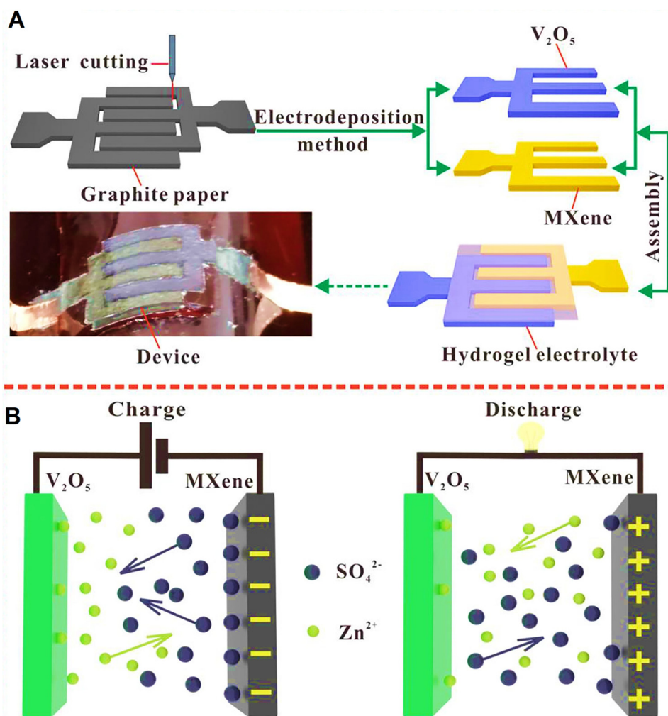
Fig. 6 (A) The design of high-performance flexible Zn-ion hybrid micro-supercapacitors using the MXene anode and \text{V}_2\text{O}_5 cathode. (B) The related mechanism of energy storage using flexible Zn-ion hybrid micro-supercapacitors (the states of charge and discharge). Reproduced with permission from ref. 96 Copyright 2021 Elsevier.
