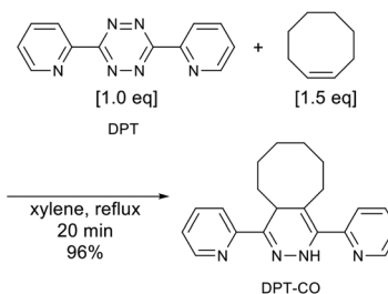
Scheme 1 Synthesis of DPT-CO from DPT and cis -cyclooctene.
