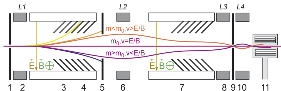
Fig. 1 Schematic overview of the ion path in the Neoma prefiling MS/MS system. (1) Entrance aperture; (2), first lens (L1) to focus; (3), first Wien filter; (4), baffles; (5), adjustable slit; (6) second lens (L2) to inverse; (7), second Wien filter; (8), third lens (L3) to focus; (9), exit aperture; (10), fourth lens (L4) to focus; (11), collision/reaction cell.
