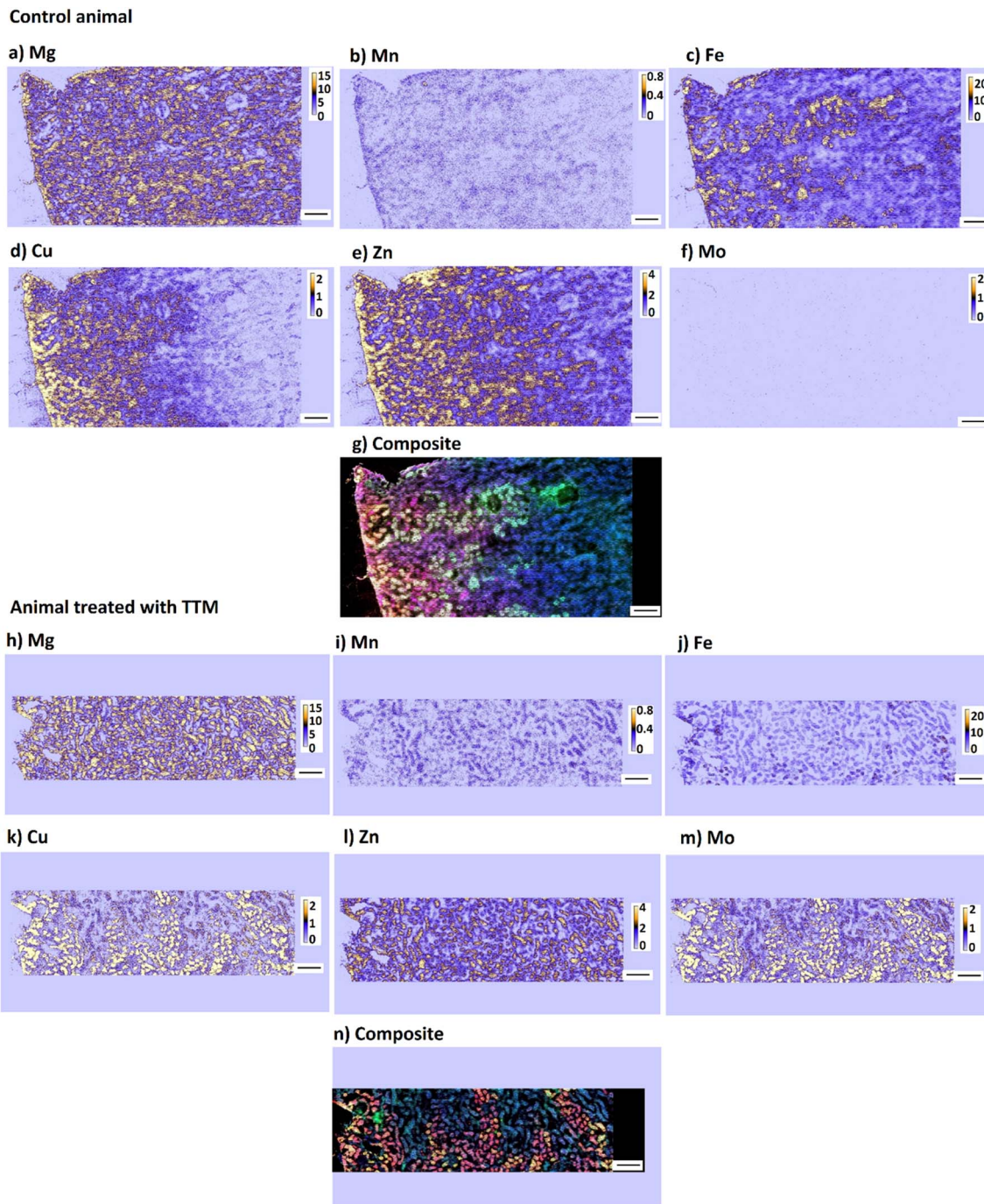
Fig. 6 Distribution of Mg, Mn, Fe, Cu, Zn and Mo (a–f, h–m), and a composite image (g, n) (red = Cu, green = Fe, blue = Mg) in rat kidney taken from a control animal (a–g) and from a rat given 60 mg per kg per day TTM (h–n) imaged at 3 \mu\text{m} resolution. The area imaged is approximately indicated in the whole-organ image in Fig. 5. Colour scale is in fg per pixel. Scale bar corresponds to 200 \mu\text{m} . The isotopes measured are ^{24}\text{Mg} , ^{55}\text{Mn} , ^{56}\text{Fe} , ^{63}\text{Cu} , ^{64}\text{Zn} and ^{98}\text{Mo} .
