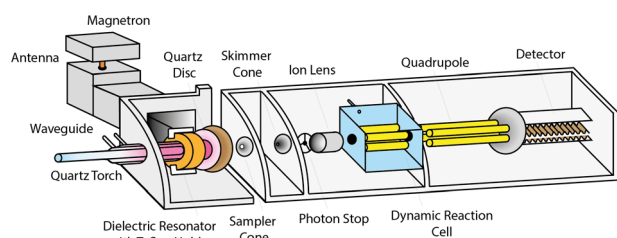
Fig. 1 Schematic depiction of the MICAP-MS.
