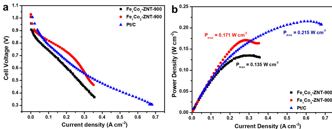
Fig. 7 (a) Polarisation and (b) power density curves obtained for Fe 1 Co 1 -ZNT-900, Fe 1 Co 2 -ZNT-900, and Pt/C cathode catalysts in H 2 /O 2 AEMFCs [anode catalyst: PtRu/C. AEM: Aemion+® 15 µm. T = 65 °C].
