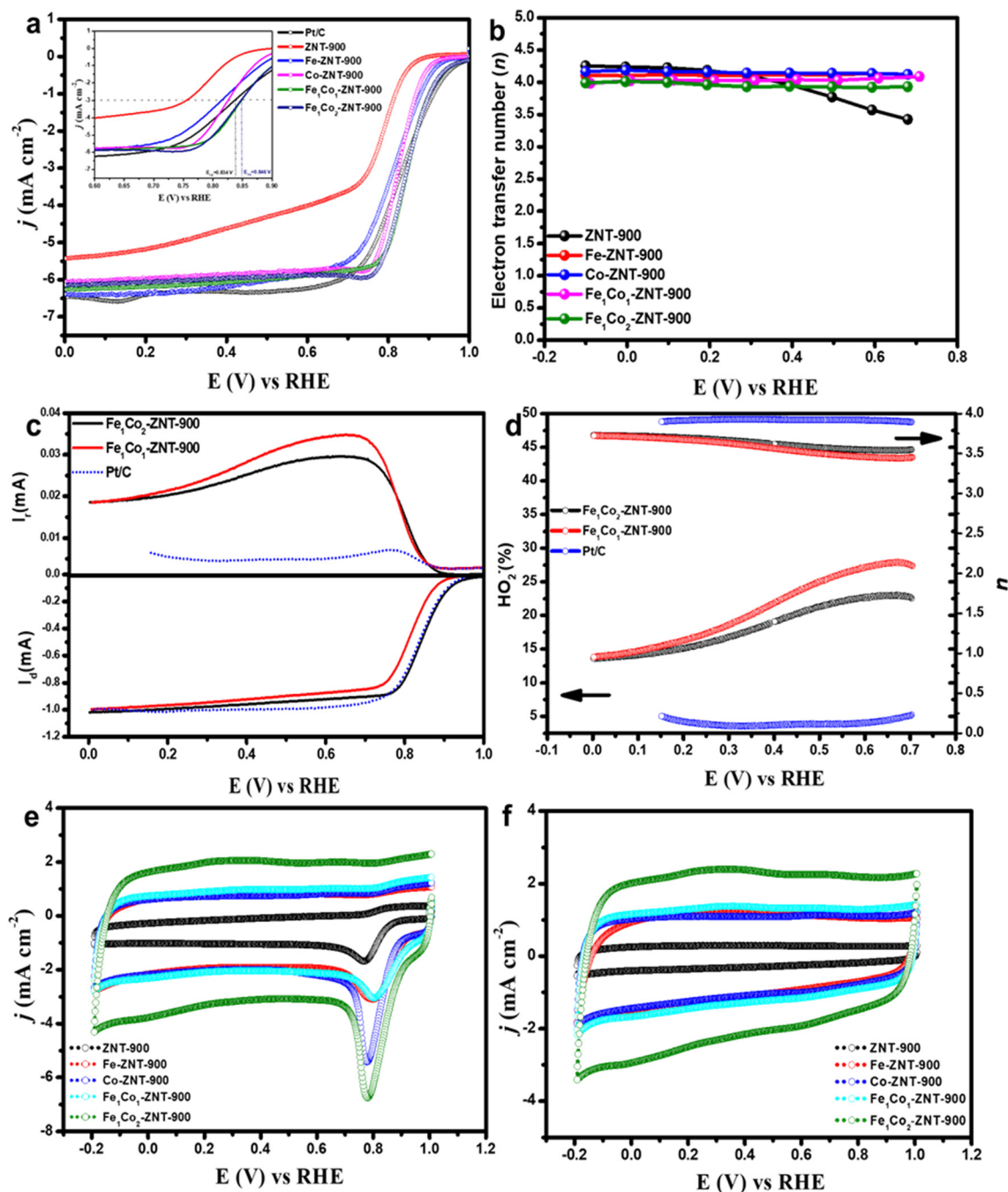
Fig. 6 (a) ORR polarisation curves for ZIF@CNT catalysts recorded at 1900 rpm with a scan rate of 10 \text{ mV s}^{-1} in O_2 -saturated 0.1 \text{ M KOH} . (b) Electron transfer number ( n ) obtained from K-L plots for all the catalysts. (c) RRDE results for Fe 1 Co 2 -ZNT-900, Fe 1 Co 1 -ZNT-900 and Pt/C catalysts in 0.1 \text{ M KOH} at 1900 rpm with a scan rate of 10 \text{ mV s}^{-1} . (d) Electron transfer number ( n ) and HO_2^- yield for Fe 1 Co 2 -ZNT-900, Fe 1 Co 1 -ZNT-900 and Pt/C catalysts. CV curves were recorded in (e) O_2 -saturated and (f) Ar-saturated 0.1 \text{ M KOH} at 100 \text{ mV s}^{-1} .
