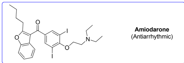
Scheme 1 Amiodarone chemical structure.
