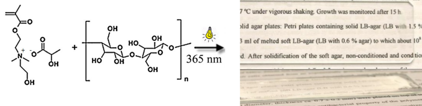
Fig. 10 Photopolymerisable cellulose coating using a cholinium-based ionic liquid methacrylate monomer as both solvent and crosslinker. Reproduced from ref. 107 with permission from the American Chemical Society, copyright 2013. A part reproduced from ref. 108 with permission from Wiley, copyright 2014.
