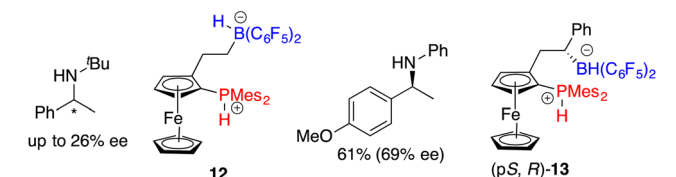
Scheme 6 Planar-chiral FLP-catalyzed asymmetric hydrogenation of imines.
