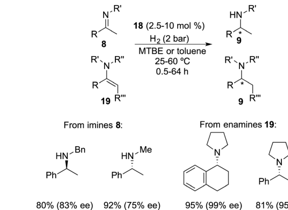
Scheme 8 Asymmetric hydrogenation of imines and enamines with ansa -ammonium borate catalysts.
