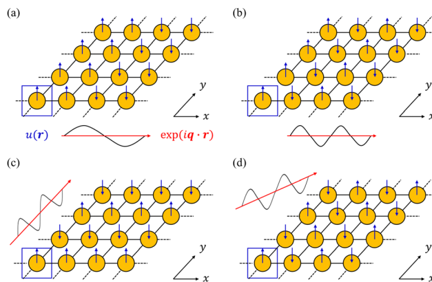
Fig. 4 Schematic illustration of how the Bloch theorem defined in eqn (5) generates four of the phonon modes of a monoatomic 2D lattice. The displacement of the atom in the primitive cell defines the cell-periodic function \mathbf{u}(\mathbf{r}) (blue), which is replicated across the other unit cells in the lattice with a phase pattern defined by plane-wave terms \exp(i\mathbf{q}\cdot\mathbf{r}) (red). In (a) and (b) the wavevector \mathbf{q} is oriented along the real-space x direction with two different wavelengths corresponding to different modulation periods. In (c) and (d), the wavevector is aligned along the y and xy directions, respectively, with the same wavelength as in (b).
