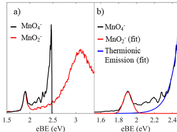
Fig. 4 Photoelectron spectrum of \text{MnO}_4^- recorded at h\nu = 2.48 eV (black), where the energy axis is in electron binding energy, \text{eBE} = h\nu - e\text{KE} . In (a) this is shown with the previously reported spectrum of \text{MnO}_2^- taken at h\nu = 3.49 eV (red) reprinted from J. Chem. Phys. , 2000, 113 , 1473, with the permission of AIP publishing. 11 In (b), a Gaussian fit to the spectral features associated with the \text{MnO}_2^- triplet state (red) is shown as well as an exponential fit to the thermionic emission (blue).
