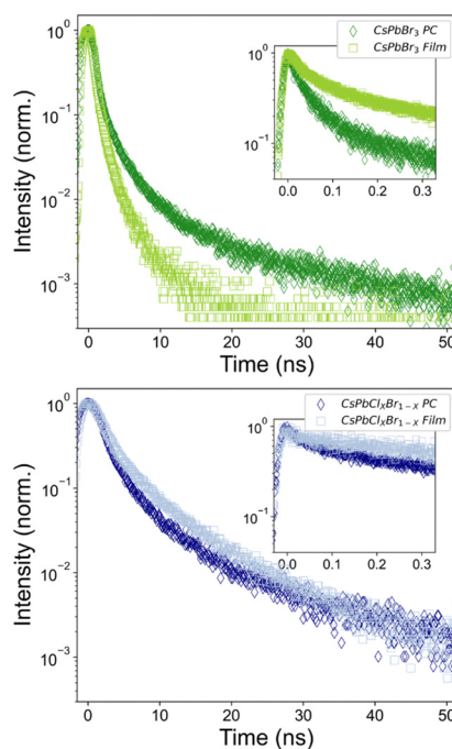
Fig. 3 Time-resolved photoluminescence (TRPL) dynamics of neat PNC films and PC C PNCs. PL decay traces of: (A) CsPbBr 3 NCs ( \lambda_{\text{ex}} = 390 nm). (B) CsPbCl 1.5 Br 1.5 NCs ( \lambda_{\text{ex}} = 350 nm).
