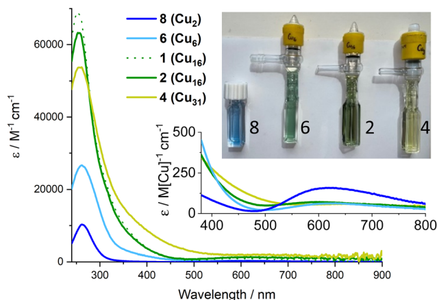
Fig. 4 UV/vis spectra of 2 , 4 , 6 & 8 reported as molar extinction coefficients. Spectra recorded at 0.1–0.4 mM[Cu] in \text{CH}_2\text{Cl}_2 (or pentane for 2 ), inset shows magnified visible region as 'per copper' normalised extinction coefficients, spectra recorded at 1.7–3.3 mM[Cu]. Photos of solutions (with [\text{Cu}] = \sim 0.24 mM).
