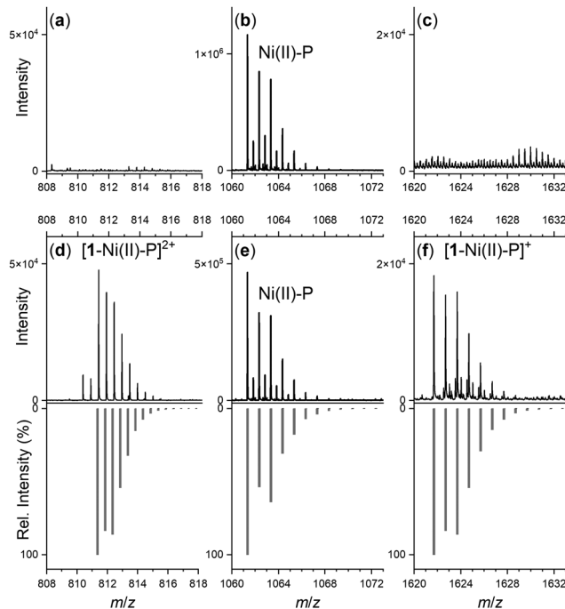
Fig. 4 Regions of the ESI-TOF-MS data from solutions of the Ni(II)-SOD peptide (Ni(II)-P) in the absence (a)–(c) or presence (d)–(f) of 1 (peptide: 1 = 1:5), showing experimental (black) or calculated (grey) signals ascribable to Ni(II)-P (b) and (e) or 1 -Ni(II)-P adducts (d) and (f).
