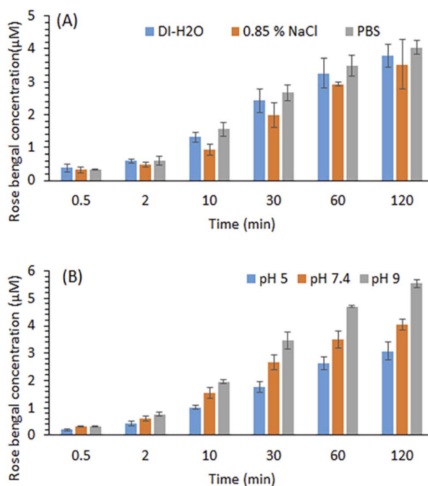
Fig. 4 Effects of ion (A) and pH in PBS (B) on the RB release from the RBiEPNs containing 0.33 wt% RB in the dark. Data is presented as mean values of triplicate measurements with \pm SD error bars.
