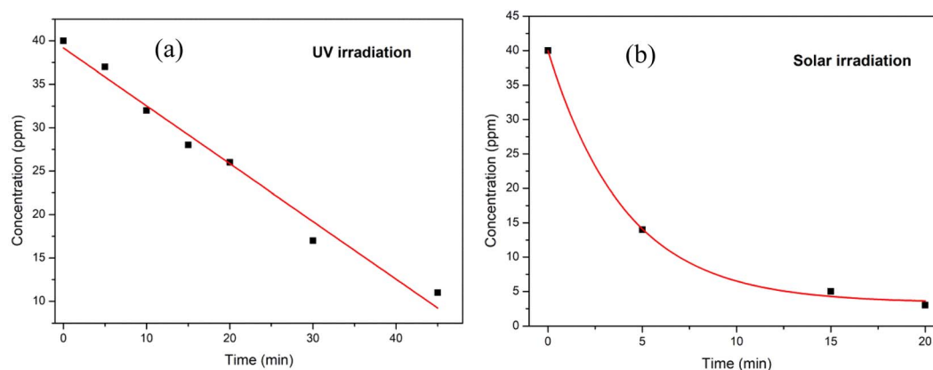
Fig. 10 Reaction kinetics model fitting for MB dye degradation under (a) UV light and (b) solar light irradiation.
