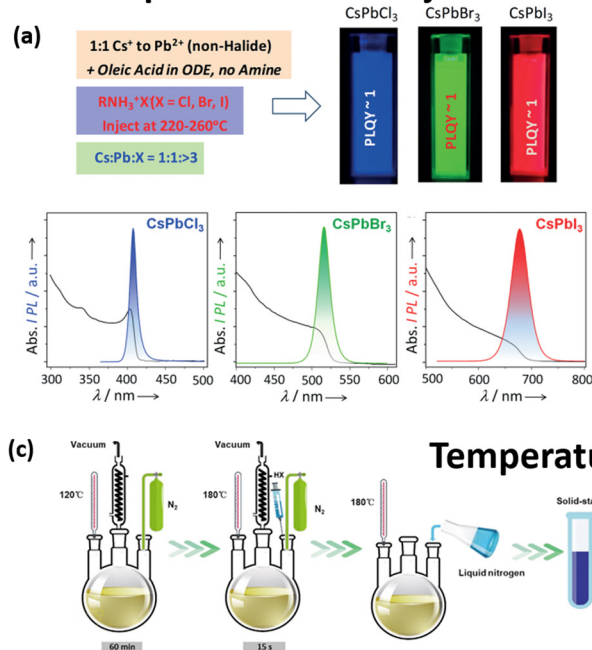
Fig. 5 (a) Schematic representation of the reaction giving near unity quantum yields in \text{CsPbX}_3 nanocrystals. Digital photographs of \text{CsPbCl}_3 (blue), \text{CsPbBr}_3 (green), and \text{CsPbI}_3 (red) nanocrystals dispersed solution under irradiation (365 nm). Absorption (black line) and corresponding PL spectra (coloured) of \text{CsPbCl}_3 , \text{CsPbBr}_3 , and \text{CsPbI}_3 nanocrystals obtained in our approach showing near unity quantum yields. Excitation wavelength was 350 nm. Reproduced with permission from ref. 112. Copyright © 2019 Wiley-VCH Verlag GmbH & Co. KGaA, Weinheim; (b) diagram showing Ni doping in \text{CsPbCl}_3 nanocrystals can boost the PLQY to near unity. Reproduced with permission from ref. 118. Copyright © 2018 American Chemical Society; (c) the schematic diagram of the synthesis method with liquid nitrogen cooling and the relationship between cooling rate and crystal quality. Reproduced with permission from ref. 131. Copyright © 2020 WILEY-VCH Verlag GmbH & Co. KGaA, Weinheim.
