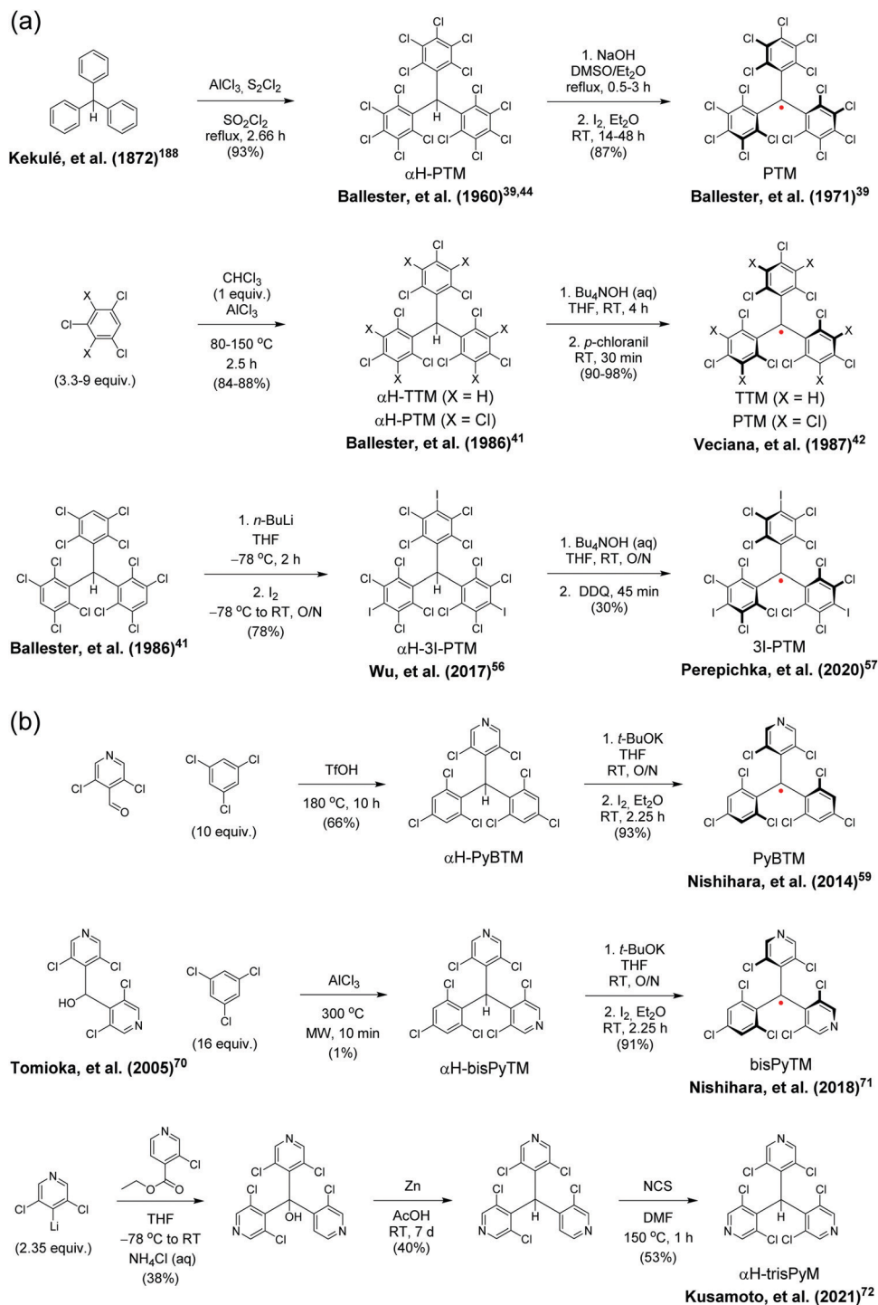
Scheme 2 Key synthetic steps for (a) TTM and PTM radicals and (b) PyBTM, bisPyTM and trisPyM radicals and their \alpha H-precurors (DDQ = 2,3-dichloro-5,6-dicyano- p -benzoquinone, NCS = N -chlorosuccinimide). Some repeating reaction steps are omitted for clarity.
