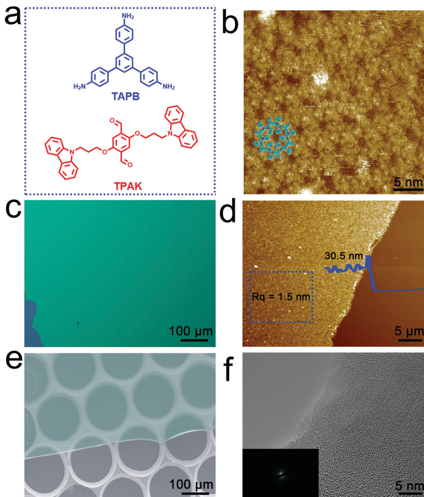
Fig. 1 (a) The chemical structure of TAPB and TPAK monomers. (b) The STM image of 2D_{\text{TPAK+TAPB}} synthesized at the octanoic acid/HOPG interface. (c) OM, (d) AFM, (e) SEM, and (f) TEM images of the 2D_{\text{TPAK+TAPB}} film synthesized at the gas–liquid interface (inset: SAED image of the 2DP film).
