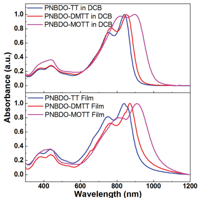
Fig. 1 UV-vis-NIR absorption spectra of the three thienothiophene-bisoxindolinylidene-benzodifurandione copolymers in DCB solutions and thin films.
