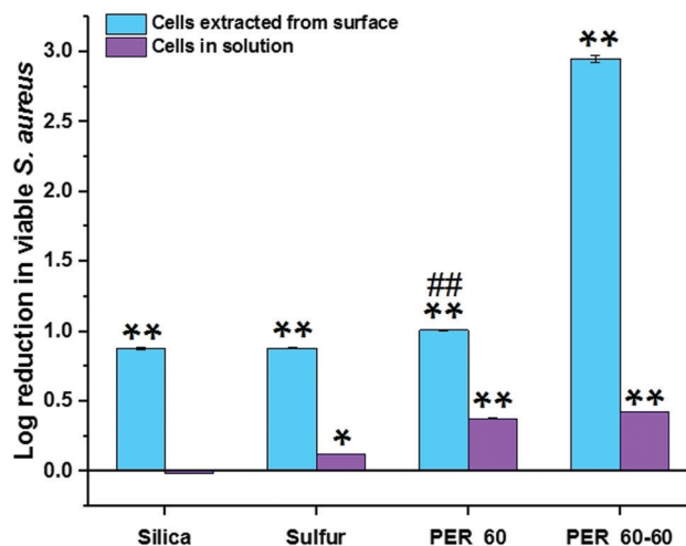
Fig. 6 A summary of the log reduction in viable S. aureus colony forming units extracted from the surface and from solution relative to uncoated glass for SiO 2 -PDMS, elemental sulfur, PER_60, and PER_60-60. * p < 0.05 relative to uncoated glass, ** p < 0.001 relative to uncoated glass and ## p < 0.001 for PER_60 compared to PER_60-60. The bacterial densities on the surface of uncoated glass and in the surrounding solution were 1.1 \times 10^7 and 1.6 \times 10^8 , respectively. All samples were tested in technical triplicate and the standard deviation was used to define the error bars.
