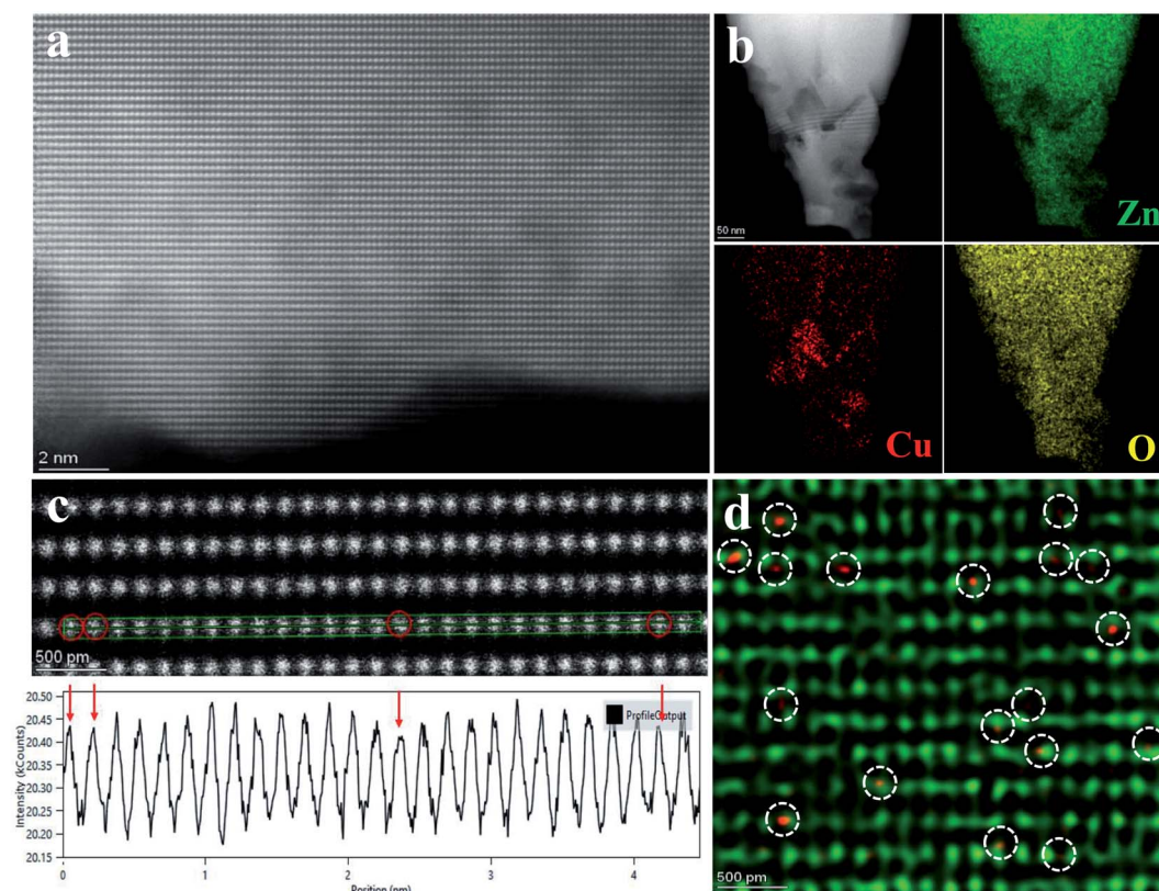
Fig. 2 (a) TEM images for Cu_1 -ZnO. (b) STEM-EDS elemental mapping of Cu_1 -ZnO. (c) Line intensity distribution diagram of Cu atoms. (d) HAADF-STEM image of Cu_1 -ZnO. The representative Cu single atom ( Cu_1 ) is indicated by the white circle.
