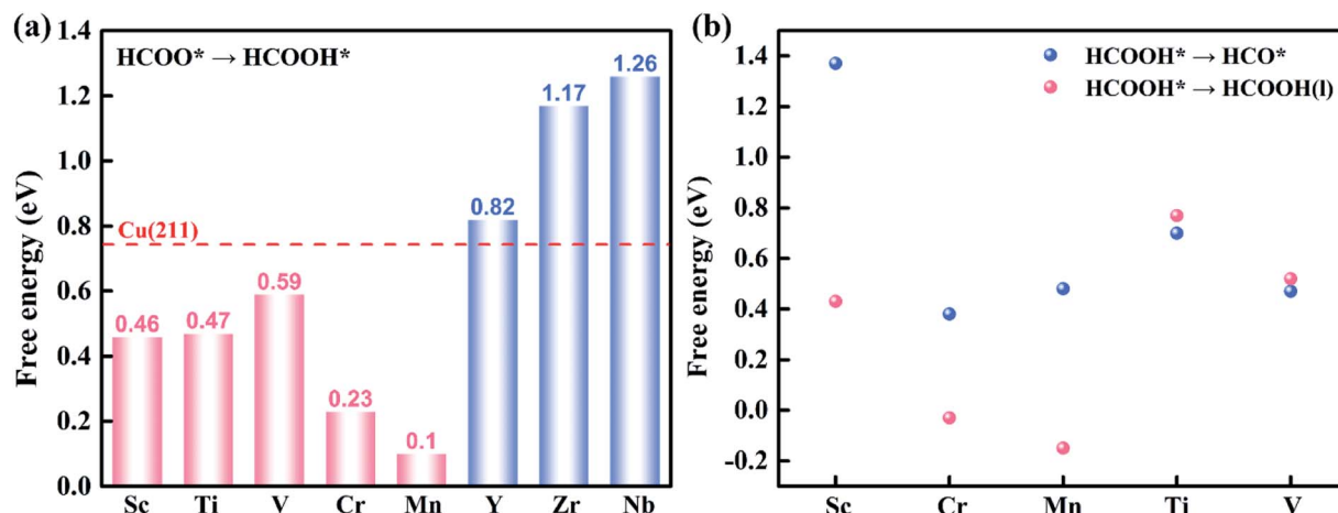
Fig. 5 (a) The \Delta G of \text{HCOO}^* + e^- + \text{H}^+ \rightarrow \text{HCOOH}^* on \text{TM@Na}_4\text{SiMo}_{12} (TM = Sc, Ti, V, Cr, Mn, Y, Zr and Nb). The screening criterion for catalytic activity is set to \Delta G < 0.74 eV (red dashed line). (b) The \Delta G for \text{HCOOH}^* hydrogenation ( \text{HCOOH}^* + e^- + \text{H}^+ \rightarrow \text{HCO}^* + \text{H}_2\text{O}(\text{l}) ) and desorption ( \text{HCOOH}^* \rightarrow \text{HCOOH}(\text{l}) + * ) on \text{TM@Na}_4\text{SiMo}_{12} (TM = Sc, Cr, Mn, Ti and V).
