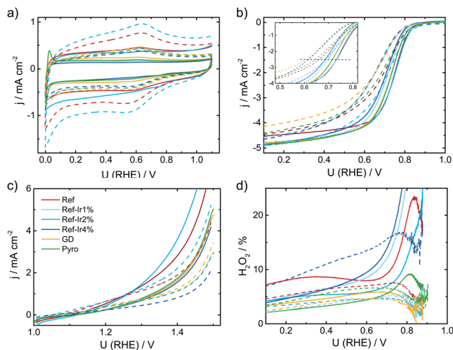
Fig. 7 Comparison of beginning of test and end of test (+10k cycles in SSC range, dashed line) electrochemical data of all investigated catalysts. (a) Cyclic voltammety in N_2 saturated 0.1 M H_2SO_4 , (b) RDE measurements in O_2 saturated electrolyte at 1500 rpm, (c) test for oxidative current density in the SSC potential range and (d) relative formation of hydrogen peroxide, determined from the RRDE measurement at 1500 rpm. All measurements performed with a catalyst loading of 0.13 \text{ mg cm}^{-2} and a sweep rate of 10 \text{ mV s}^{-1} .
