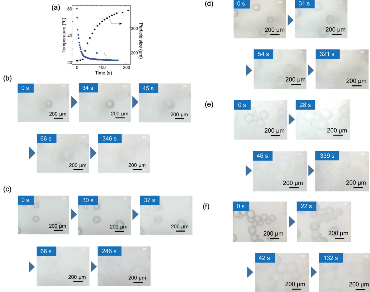
Fig. 7 (a) Variation in the diameter and temperature of the spherical PNIPA gel with time during a temperature jump from 60 °C to 20 °C, (b)–(f) Optical microscopy images in a temperature jump from 60 °C to 20 °C for (b) PNIPA gel, (c) PNIPAA 0.9 - b -PDMA 0.1 gel, (d) PNIPAA 0.8 - b -PDMA 0.2 gel, (e) PNIPAA 0.7 - b -PDMA 0.3 gel, and (f) PNIPAA 0.8 - r -PDMA 0.2 gel.
