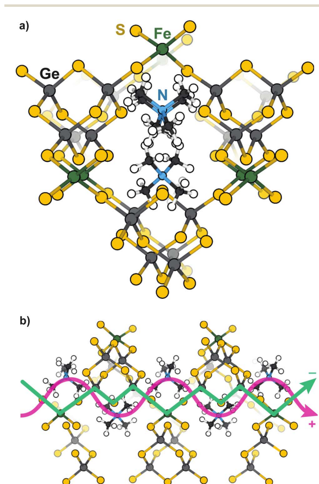
Scheme 1 Representations of \text{TMA}_2\text{FeGe}_4\text{S}_{10} viewed along the (a) [100] and (b) [010] directions. Proposed conduction pathways of delocalized electrons and extra-framework cations are highlighted in green and pink, respectively.
